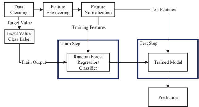
Fig. 1. The Main Components in Our Proposed Model
